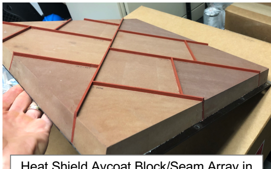
Heat Shield Avcoat Block/Seam Array in Combined Convective/Radiant Heating
