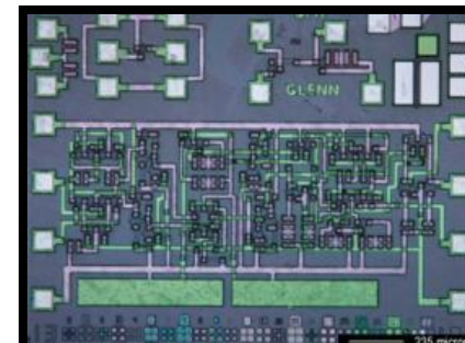
High Temperature Signal Processing and Wireless
