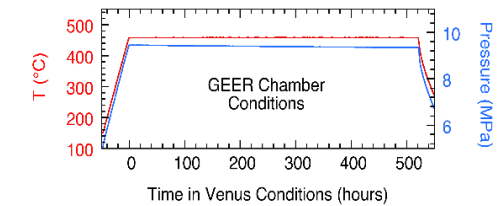
High Temperature Ring Oscillator Continues Stable Operation in these Venus Simulated Conditions for 521 hours
