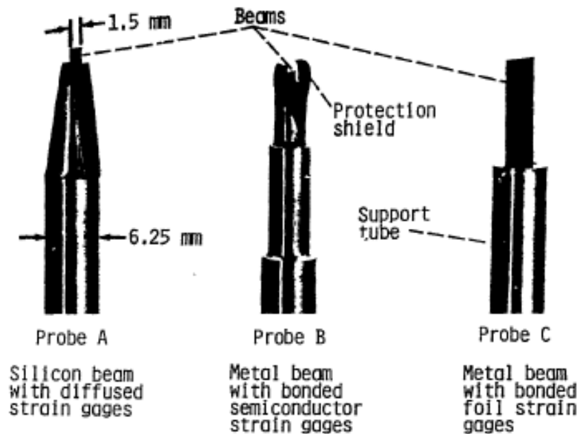
Figure 1. - Drag-Force anemometers.
