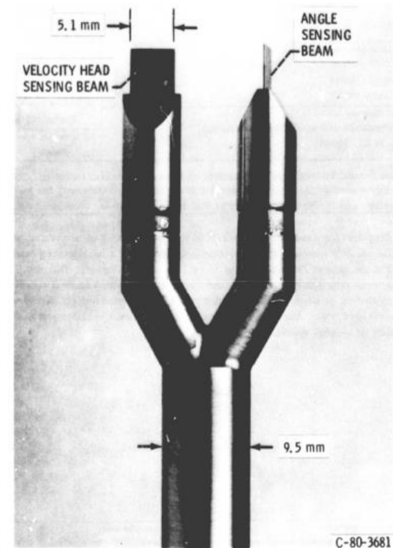
Figure 11. - Unsteady flow angle probe for use in turbofan engine inlet.
