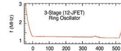
High Temperature Ring Oscillator Continues Stable Operation in these Venus Simulated Conditions for 521 hours
