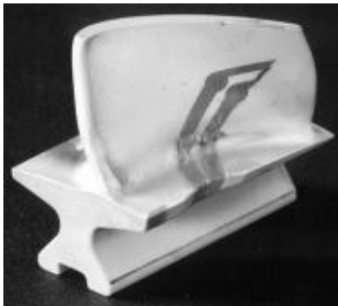
PdCr strain sensor to T=1000^{\circ}\text{C}
